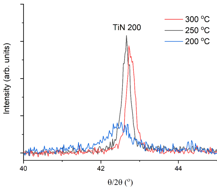
Figure 1: \theta/2\theta XRD diffractogram of the 200 reflection of TiN deposited with PEALD at three different temperatures. The deposition temperature improves the crystallinity.
