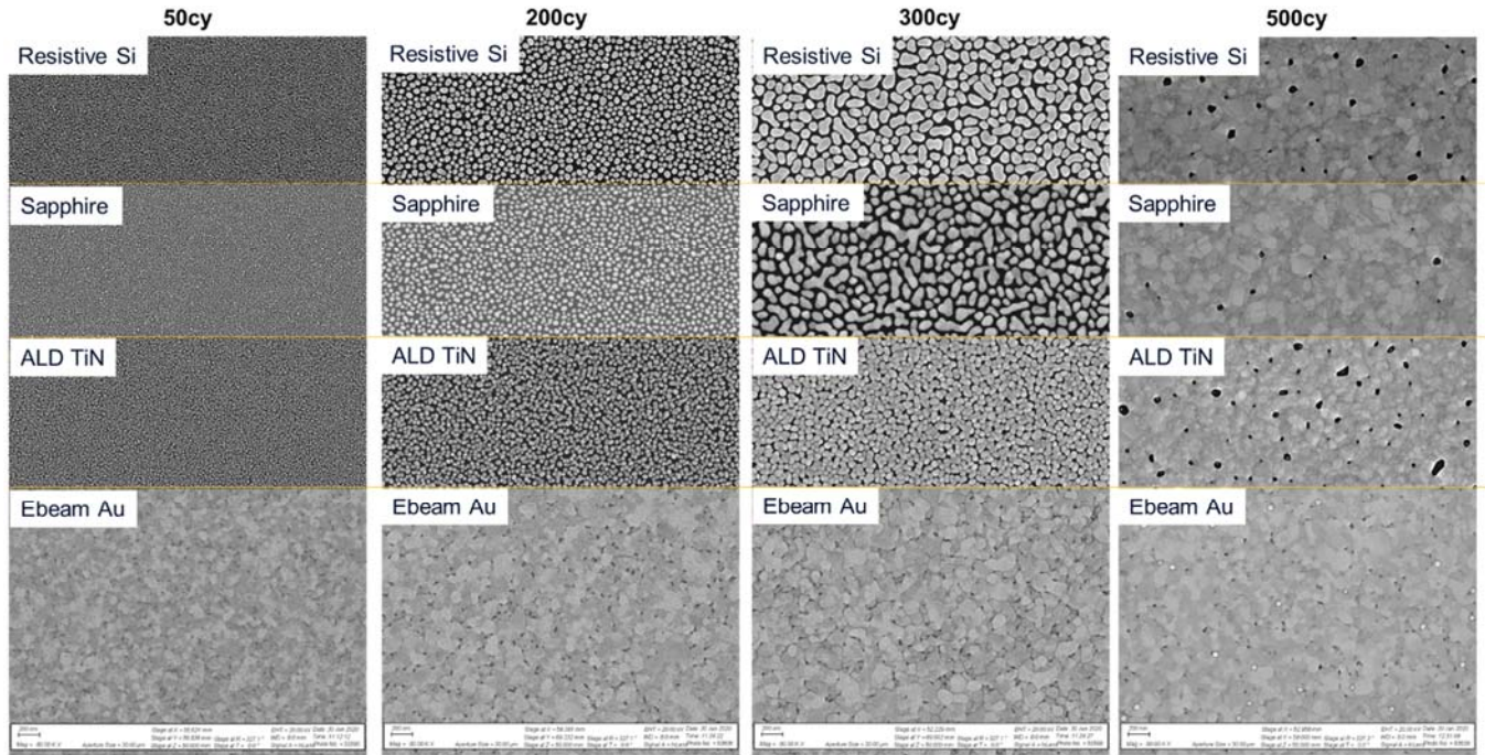
SEM images showing the evolution of ALD Au on various substrates with increasing number of cycles
