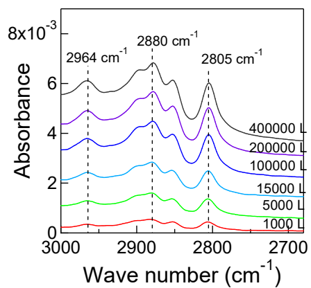
Fig. 1 IR absorbance spectra measured from the TDMAS adsorbed surface.
