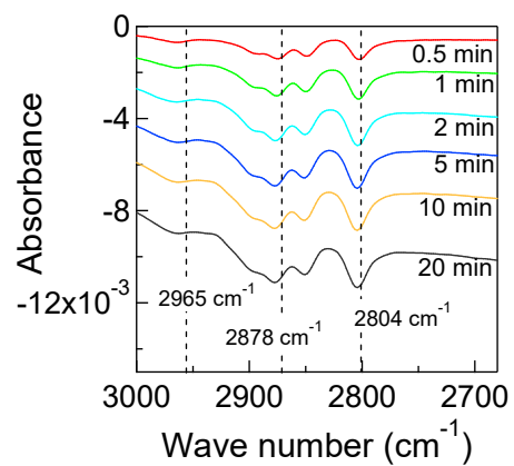
Fig. 2. IR spectra measured from the TDMAS adsorbed surface with a plasma-excited ammonia treatment.
