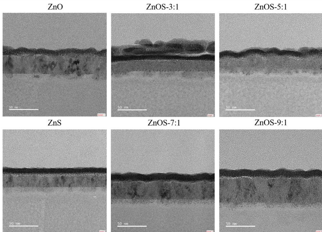
Fig. 2 TEM images of ZnO, ZnS and Zn(O,S) films with different ratios
