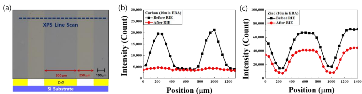
Figure 1 (a) XPS line scan of patterned ZnO OM image. (b) and (c) Carbon and zinc peak intensity position on the patterned ZnO before and after RIE.
