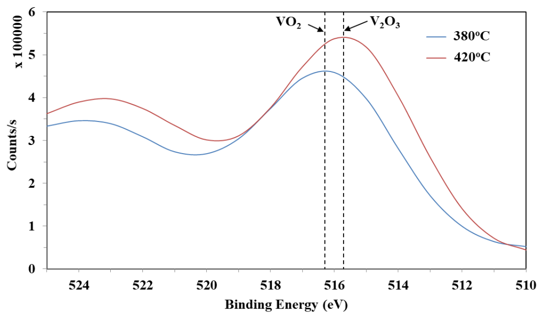
Figure 1. The XPS spectra of vanadium oxides deposited at 380°C and 420°C.
