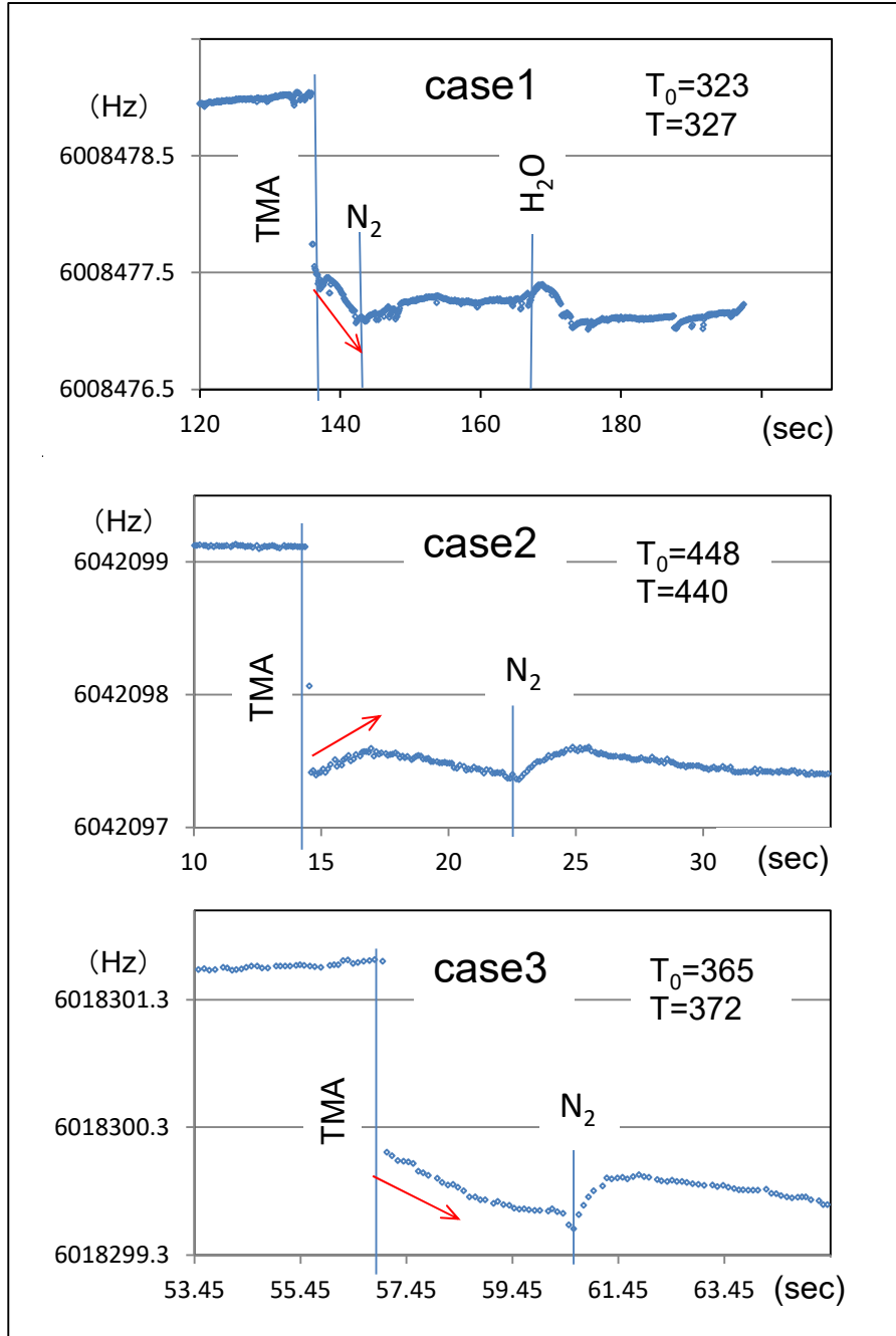
Fig.2 transient response after TMA dose
