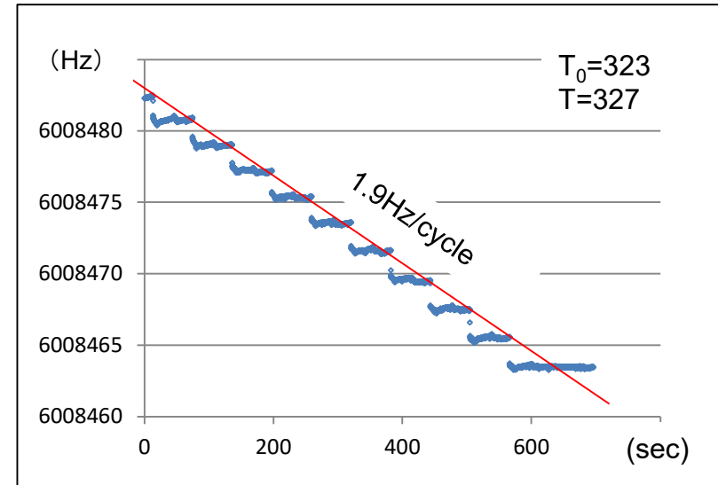
Fig.3 LCM frequency envelope of TMA/ H_2O
