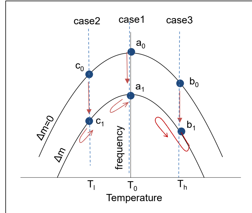
Fig.1 f-T diagram of Langasite crystal
