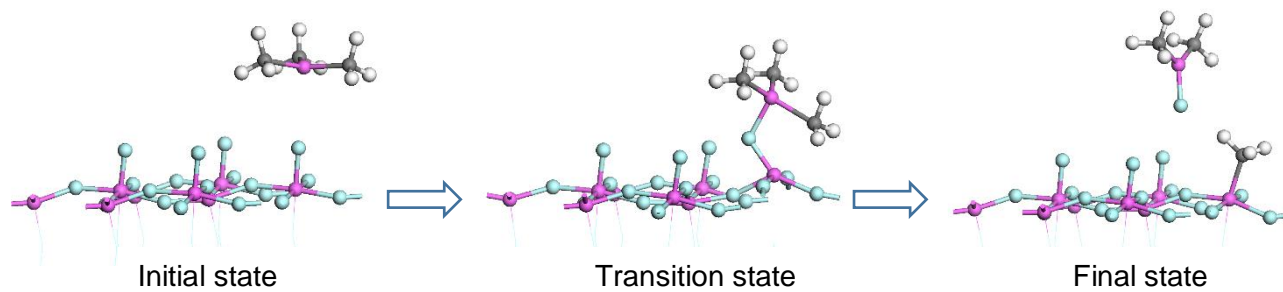
Fig.1 DFT-calculated pathway for the ligand-exchange reaction between \text{Al}(\text{CH}_3)_3 and \text{AlF}_3 .
