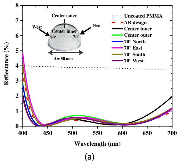
Figure 1. (a) Measured reflection spectra of the centre positions of the outer and inner surfaces of the PMMA dome and at 70° inclined positions in four directions from the centre on the outer surface exhibit excellent 3D conformality of ALD coatings. (b) Adhesive films on double-sided antireflection coated PMMA even after climate test.
