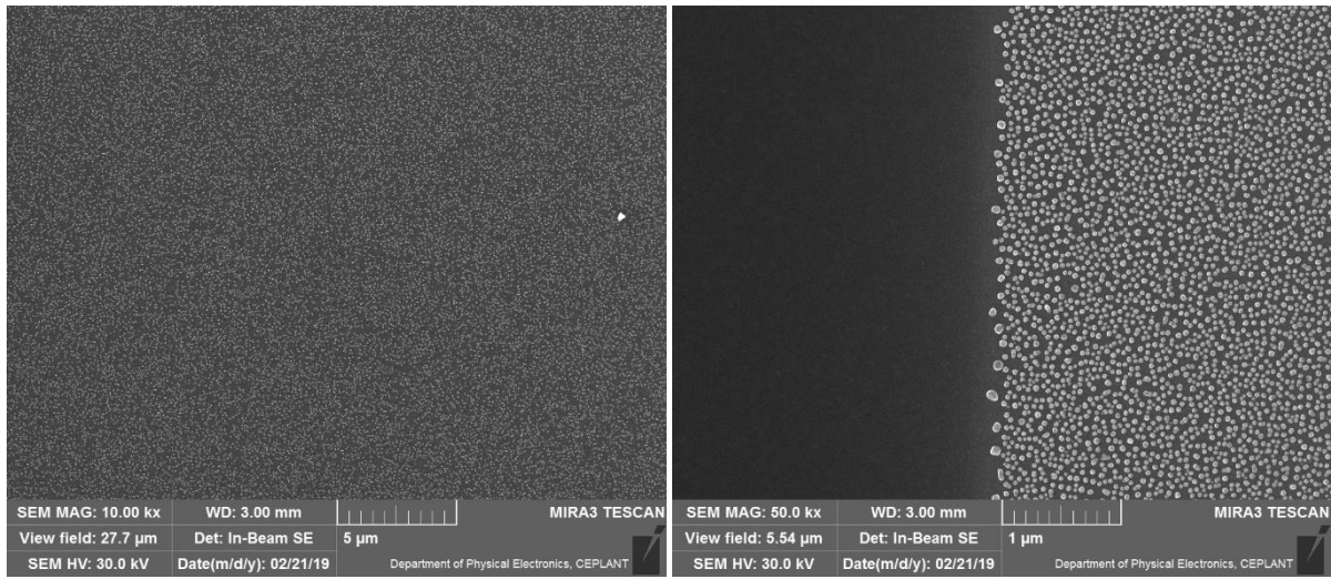
Figure 1: SEM images of a layer of CuCl crystallites on a silicon substrate cleaned by RCA protocol.
