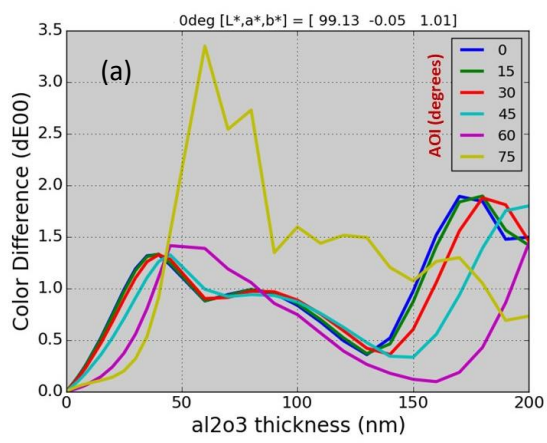
Figure-1: Color difference from uncoated silver as a function of Al 2 O 3 coating thickness for AOI=0-75°. (a) 99.9% Silver: \Delta E_{00} < 1 for AOI=0-60° at Al 2 O 3 thickness 80-130nm; (b) Silver with 5% Cu: no \Delta E_{00} < 1 for AOI=0-60° except for sub 10nm Al 2 O 3
