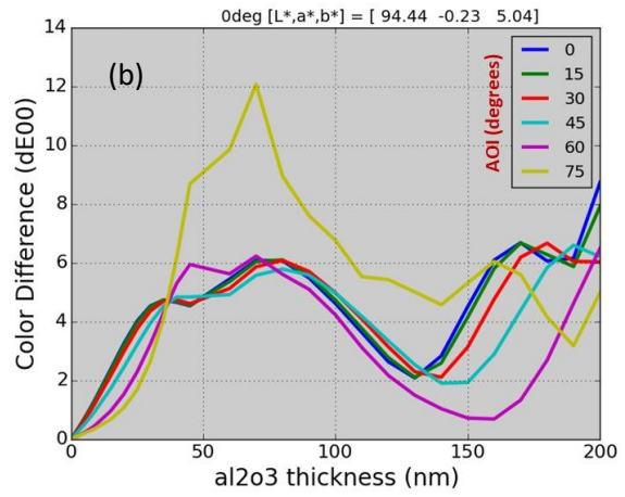
Figure-1: Color difference from uncoated silver as a function of Al 2 O 3 coating thickness for AOI=0-75°. (a) 99.9% Silver: \Delta E_{00} < 1 for AOI=0-60° at Al 2 O 3 thickness 80-130nm; (b) Silver with 5% Cu: no \Delta E_{00} < 1 for AOI=0-60° except for sub 10nm Al 2 O 3
