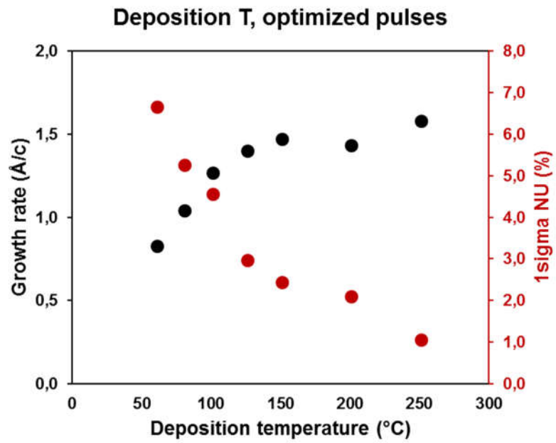
Figure 1. The effect of deposition temperature on growth rate and film thickness uniformity on the single wafer SiO 2 process.
