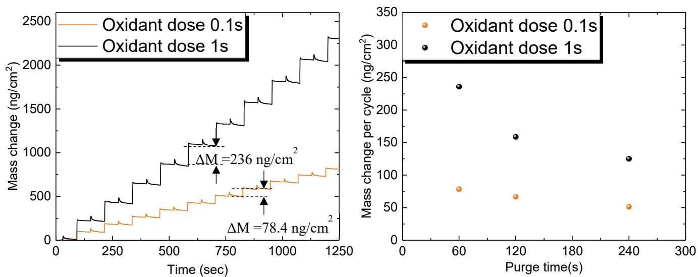
Fig.1 QCM mass change measured during o-MLD at 100 °C with variable oxidant doses and a 2s EDOT dose. Left figure illustrates raw QCM mass change data with 60s purge time and left figure shows GPC versus purge time for two oxidant exposures.
