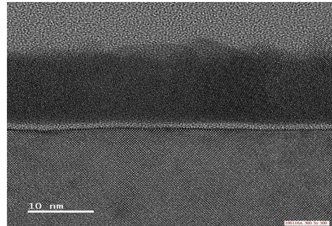
Fig.4-TEM close look of In 2 O 3
