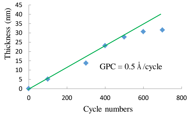
Fig.1-GPC curve of In 2 O 3
