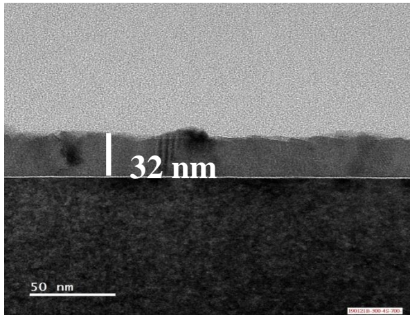
Fig.3-TEM image of cross section
