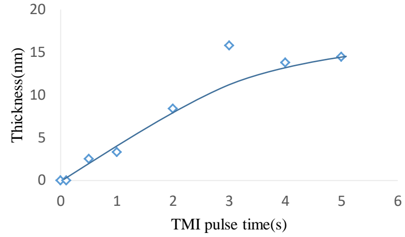
Fig.2-Saturation curve of In 2 O 3 (300 cycle numbers)
