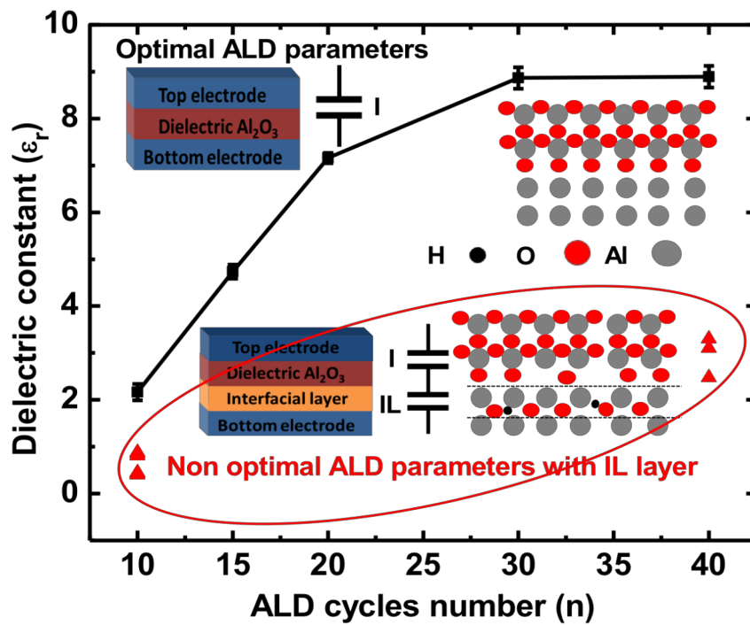
Figure: Variation of the dielectric constant with ALD cycles number for Al/Al 2 O 3 /Al trilayer fabricated using both optimal and non-optimal ALD condition. The schematics show the difference in metal-insulator interface using two different ALD conditions
