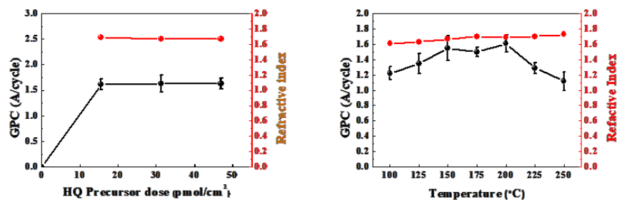
Figure 1. Growth of MLD indicone (left) HQ pulse time dependence (right) growth temperature dependence
