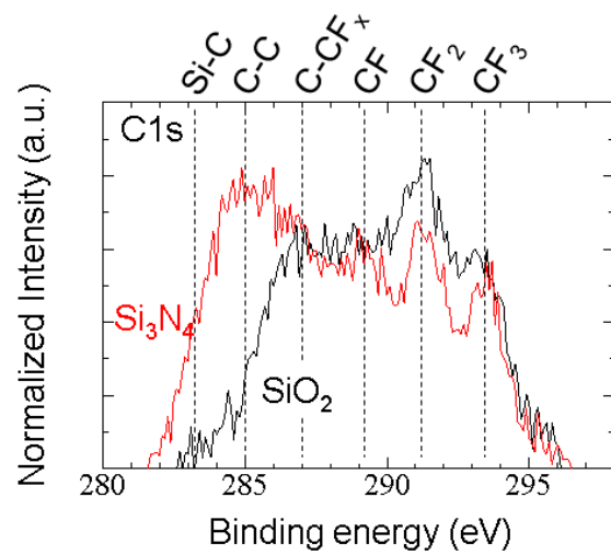
Figure 1. C 1s XPS spectra of SiO 2 and Si 3 N 4 after fluorocarbon deposition.
