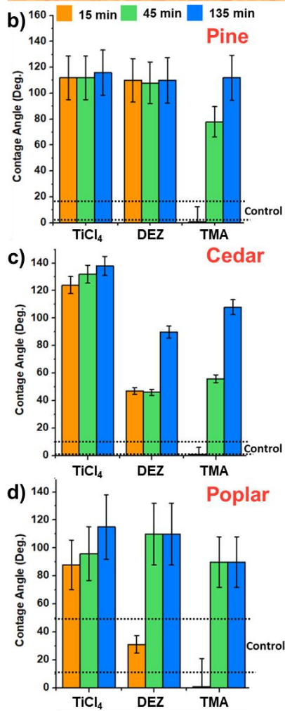
Fig. 3: Capillary face water contact angle for wood blocks as a function of ALD precursor and exposure time (15, 45, 135 minutes). a) shows the reference cut capillary face and capillary draw direction relative to the contact angle drop. Data was collected for b) Pine c) Cedar and d) Poplar wood species. Error bars represent the sample to sample standard deviation for untreated wood blocks. Dotted black lines show the range of contact angles obtained for untreated wood.
