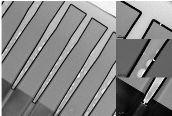
Figure 2. TEM images of the HfO 2 deposited at 400 °C using the CMENHa
