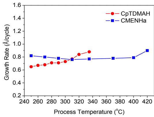
Figure 1. Thermal ALD windows of the CMENHa and CpTDMAH
