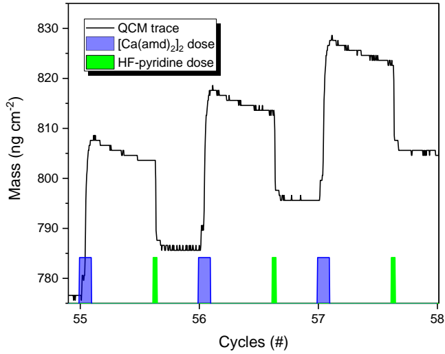
Figure 1: QCM response during the growth of high quality CaF 2
