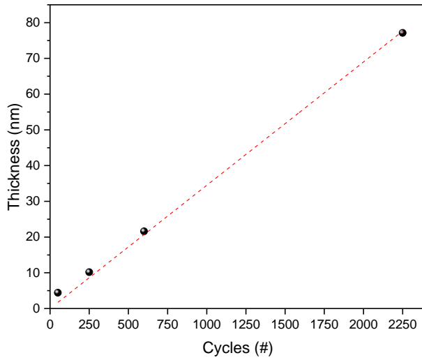
Figure 2: Thickness of CaF 2 thin films vs. applied number of cycles. The dashed line serves to guide the eye.
