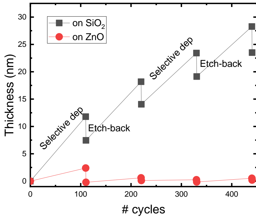
Figure 1. SiO 2 film thickness as a function of the number of cycles on growth (SiO 2 ) and non-growth (ZnO) areas. After every 110 selective ALD cycles, an etch-step is inserted to remove unwanted deposition on the non-growth area. The entire process is cycled to reach extreme selectivity.
