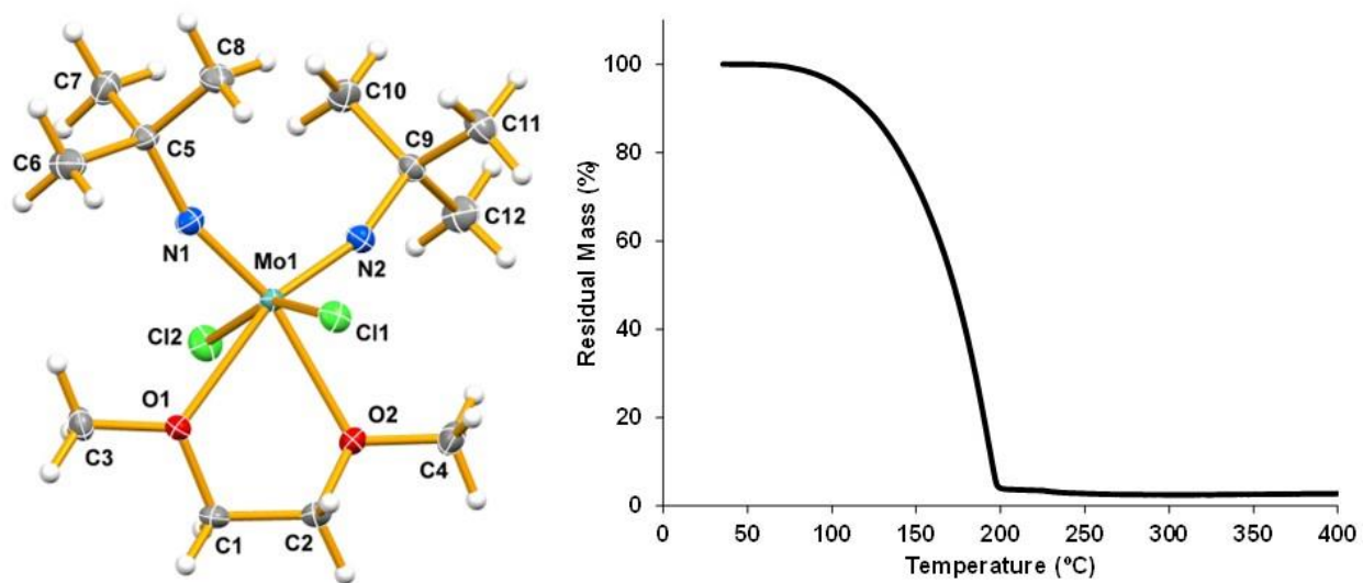
Figure 1. Solid-state structure of bis(tert-butylimido)molybdenum(VI)dichloride-(1,2-dimethoxyethane) (left) and thermal gravimetric analysis of the same compound (right). The thermal ellipsoids are drawn at the 50% probability level and the TGA ramp rate is 10 °C/min.
