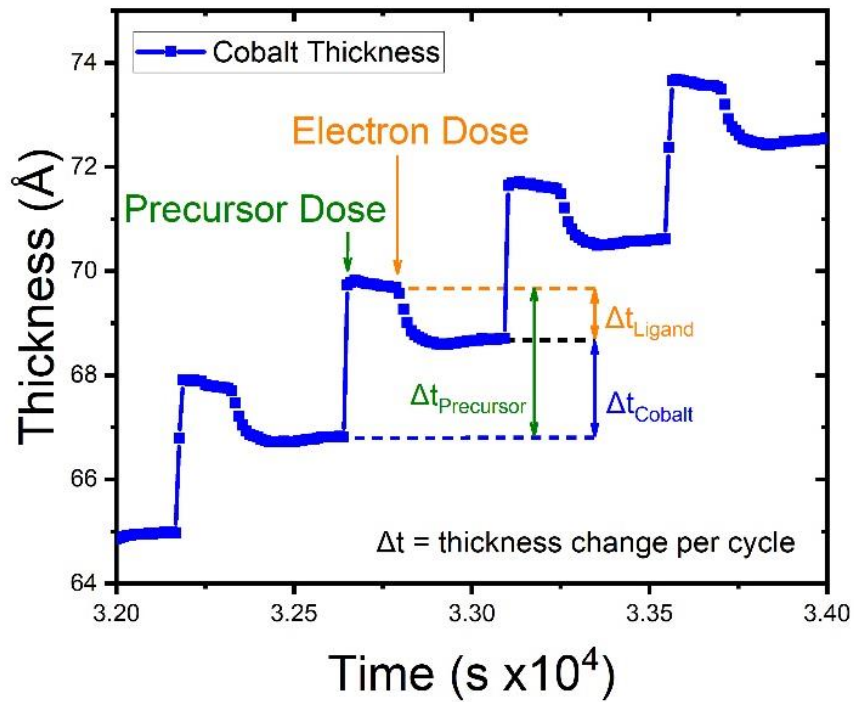
Figure 1. Real-time in situ ellipsometry of cobalt thickness during 4 EE-ALD cycles.
