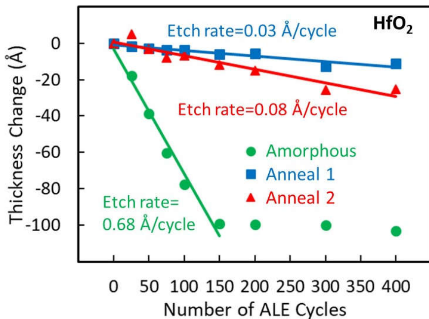
Supplemental Figure 1. ALE for three different hafnium oxide films using HF and DMAC at 250 °C. The Anneal 1 and 2 films are polycrystalline HfO 2 . The amorphous film was completely etched after 150 cycles.
