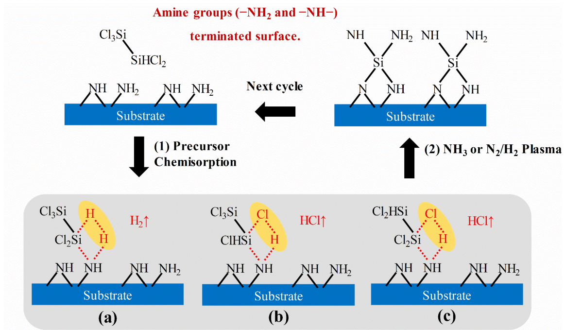
Figure 2. Schematic of the proposed surface reaction pathways of SiN x PEALD using PCDS on amine groups (-NH 2 and -NH-) terminated surface.
