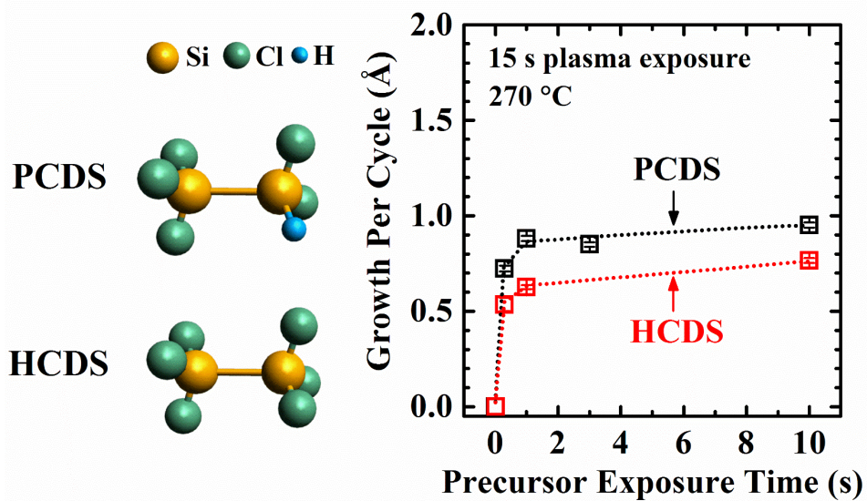
Figure 1. Schematic of the molecular structures of PCDS and HCDS and comparison of the saturation curves of GPC as a function of precursor exposure time.
