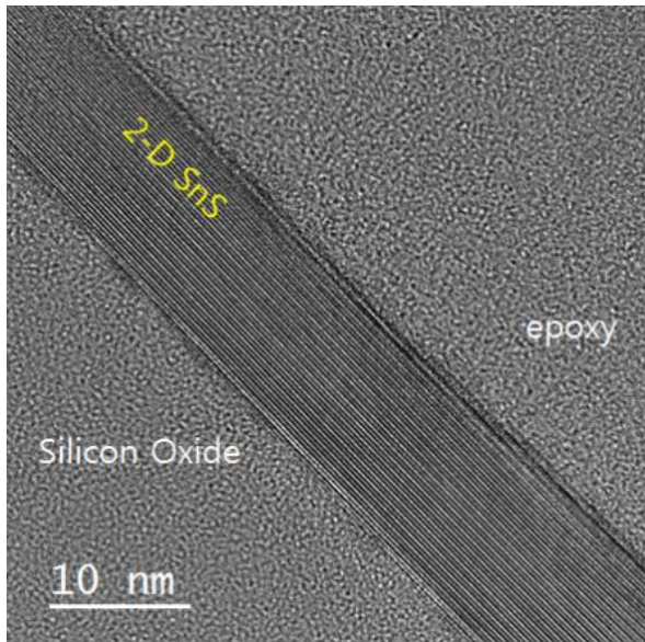
Figure 1. HRTEM images of the SnS film grown at 240 °C
