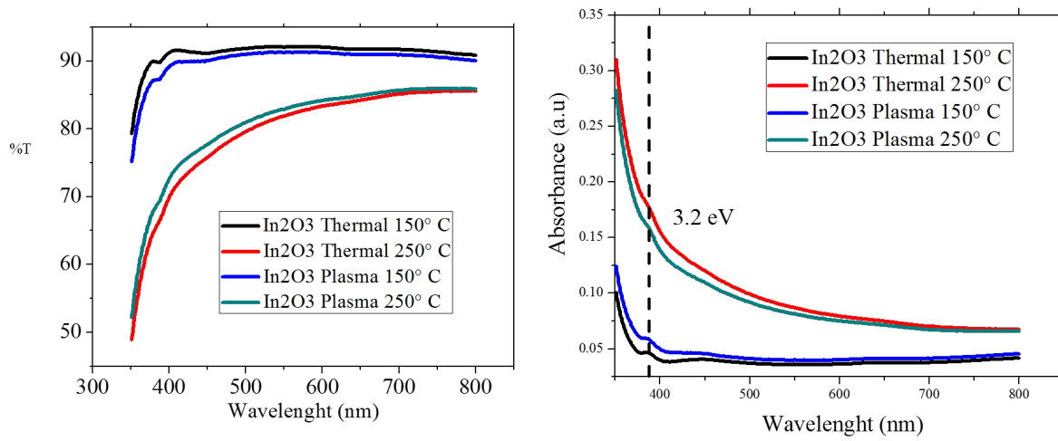
Figure 1 transmittance and absorbance spectra of In 2 O 3 obtained by ALD thermal and PEALD at 150 and 250 °C on a glass substrate.
