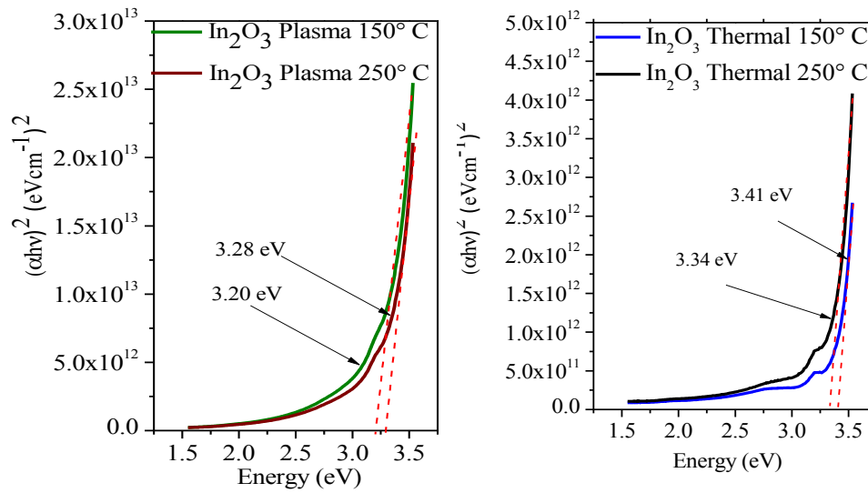
Figure 2 Tauc plot of In 2 O 3 by PEALD at 150°C and 250°C plasma and thermal deposition respectively.
