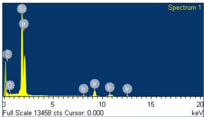
Figure 2. EDS analysis of Ir thin films on Si (100) substrates.
