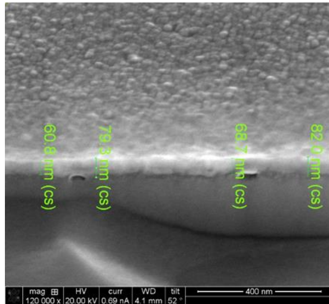
Figure 1. FE-SEM micrograph of ALD Ir film on Monel K-500 steel alloy cross-sectioned by FIB.
