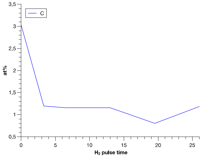
Carbon content vs H 2 pulse time
