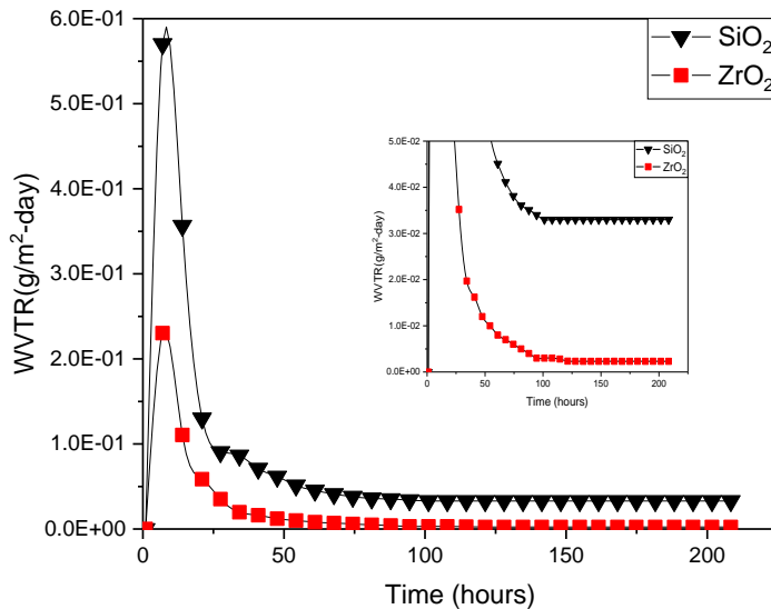
<Fig.3. WVTR characteristics of ZrO 2 &SiO 2 encapsulation layer >
