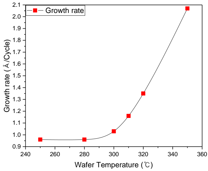
<Fig.1. ALD window of CpZr(DMA) 3 >
