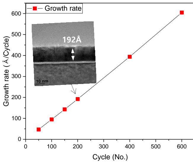
<Fig.2. Linearity of CpZr(DMA) 3 at 250°C >
