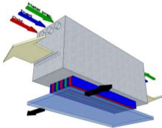
Figure 1: Schematic of a close-proximity open air SALD gas manifold, where the precursor gas channels are separated by inert gas channels.
