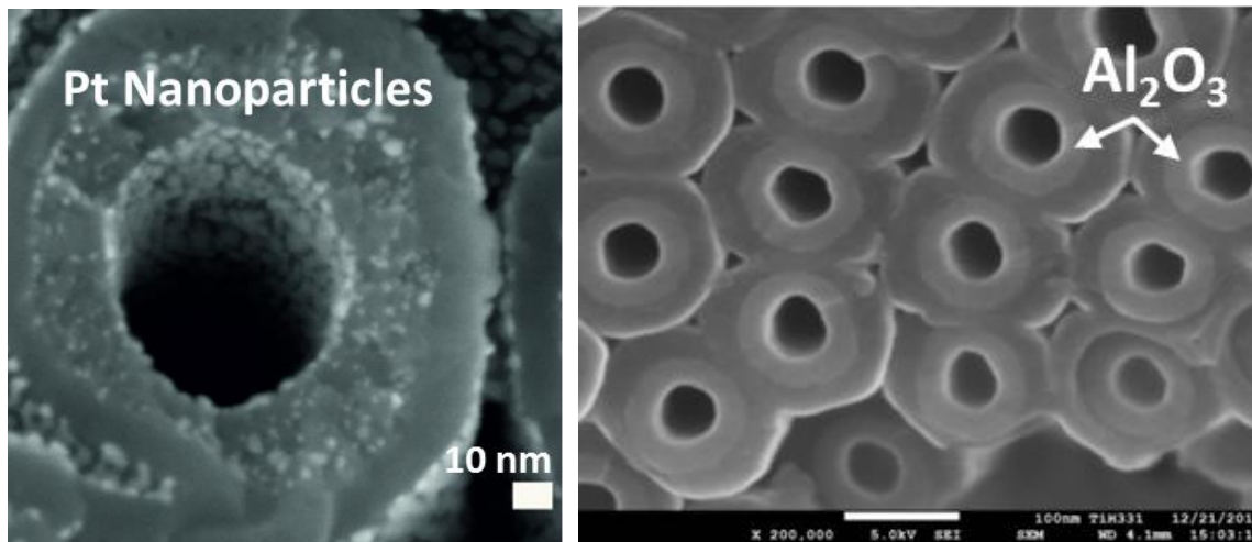
Figure 1: (Up) Bottom part SEM image (left) and cross section STEM-HAADF image (right) of 5 \mu\text{m} thick TiO 2 nanotube layers coated with crystalline ZnO coating [8]. (Down) Bottom parts SEM images of 5 \mu\text{m} thick TiO 2 nanotube decorated with Pt nanoparticles (left), and 20 \mu\text{m} thick TiO 2 nanotube coated with amorphous Al 2 O 3 coatings (right).
