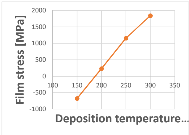
Figure 1. Measured stress of \text{HfO}_2 film on silicon substrate as a function of the ALD temperature.
