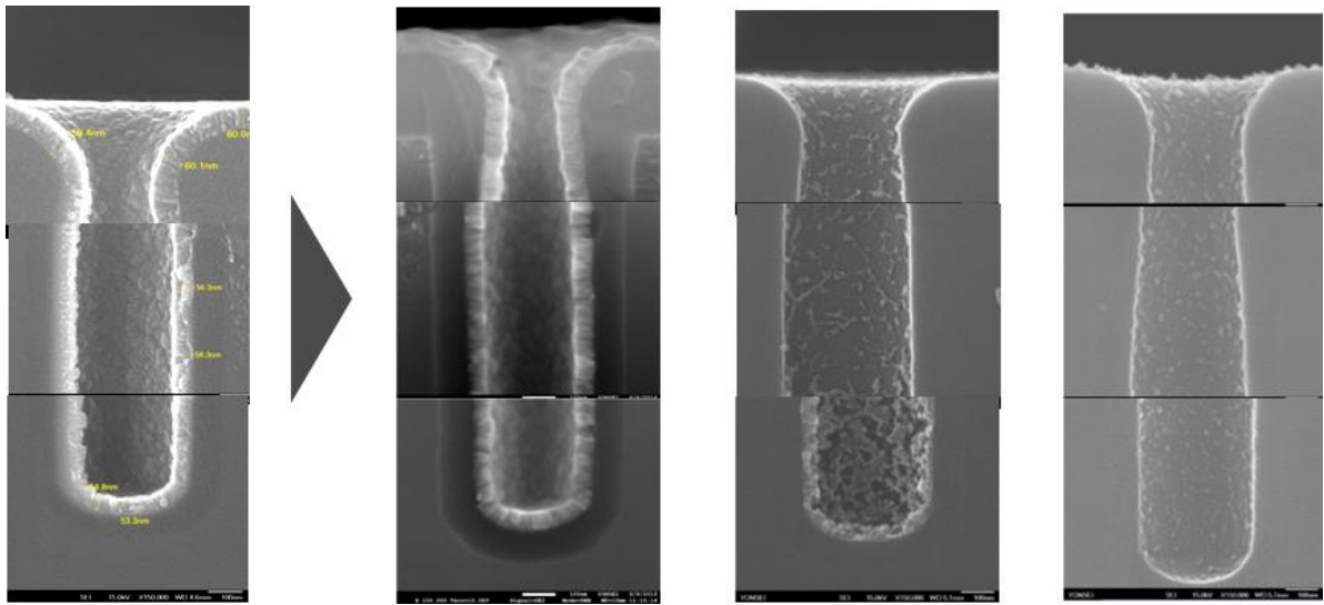
Figure 1. SEM image of thermal etching of ZrO_2 deposited in patterned wafer
