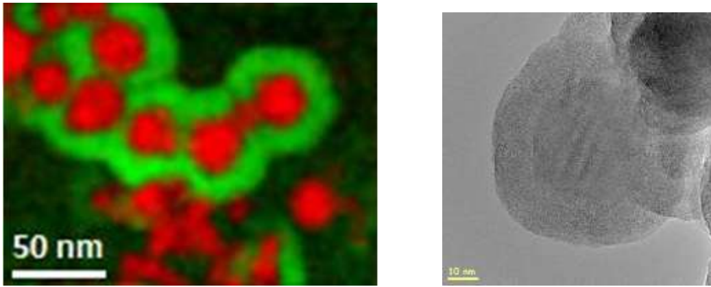
Figure 1. TEM-EDX map and HRTEM micrograph of \text{Fe}_3\text{O}_4 (red)/ \text{TiO}_2 (green) core-shell nanoparticles.
