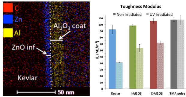
Figure: TEM-EDX map of a cross section of a processed Kevlar fiber (left) and comparison of the toughness moduli of various samples before and after UV irradiation (right).
