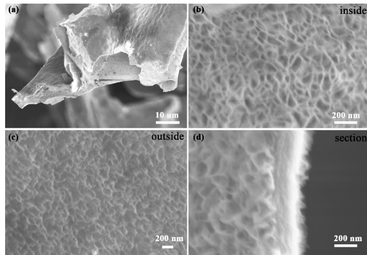
Fig. 2. SEM images of as-prepared 3D porous carbon.
