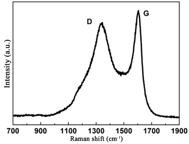
Fig. 1. Raman spectrum of as-prepared 3D porous carbon.
