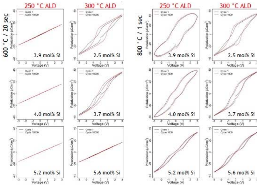
Figure 2. FE characteristics of FeRAM devices with various mol % Si and RTP conditions.
