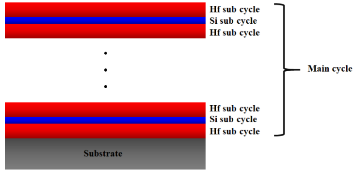
Figure 1. Schematic diagram of Si:HfO 2 deposition method. Hf sub-cycle means HfO 2 sub-cycle, and Si sub-cycle means SiO 2 sub-cycle, respectively.
