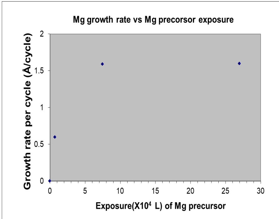
Figure 1. Self-limiting behavior of Mg (CPET) 2 exposure
