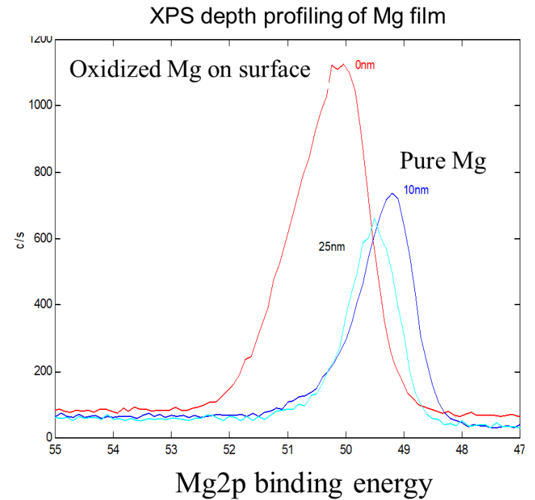
Figure 2. XPS depth profiling of Mg film (~70nm).
