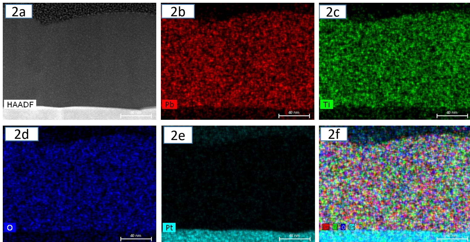
Figure 2: (a)Detail STEM image of ALD PTO coated Pt film with corresponding EDS elemental maps for Pb (b), Ti (c), O (d), Pt (e), and combined (f)
