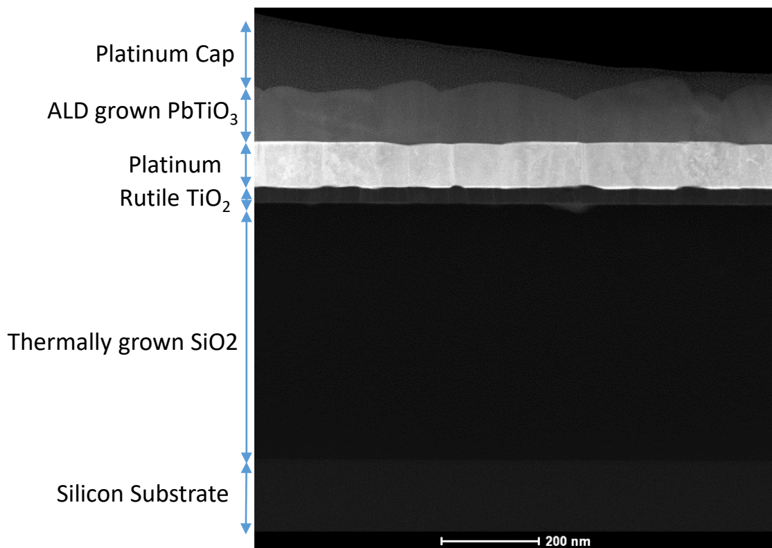
Figure 1: STEM image of ALD PbTiO 3 coated platinum lower electrode stack. Films from bottom to top: Si Substrate, SiO 2 , TiO 2 , Pt (brightest layer), PTO (rough layer), Pt capping layer
