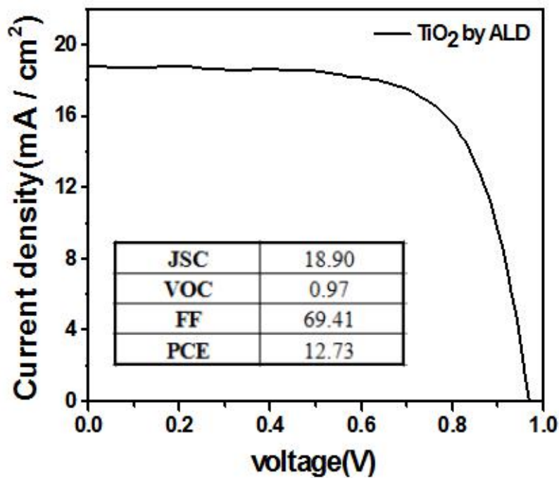
Fig.2. J-V curves of a small PSC ( 0.045 \text{ cm}^2 ) determined under simulated AM 1.5 G illumination and the corresponding photovoltaic parameters.
