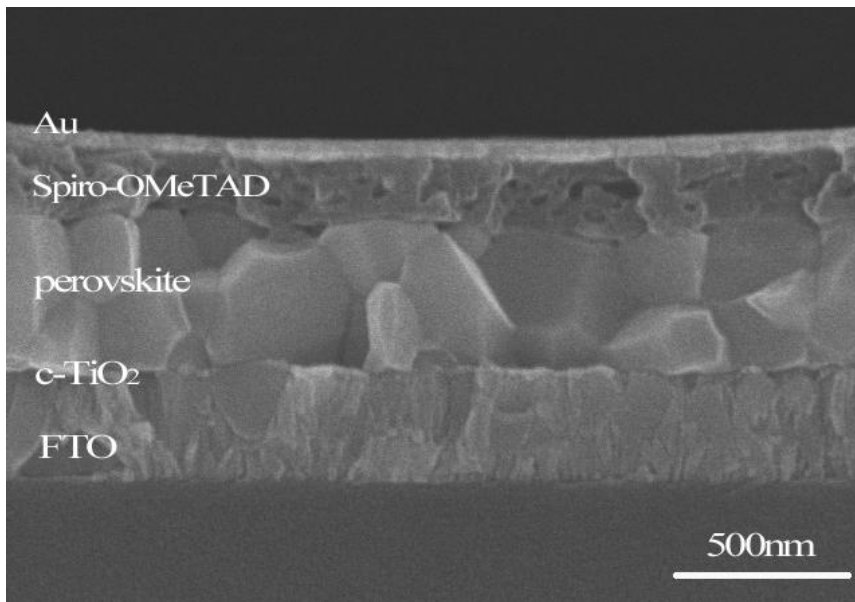
Fig.1. Device structure and cross-sectional scanning electron microscopy (SEM) image of planar perovskite solar cells (PSCs).
