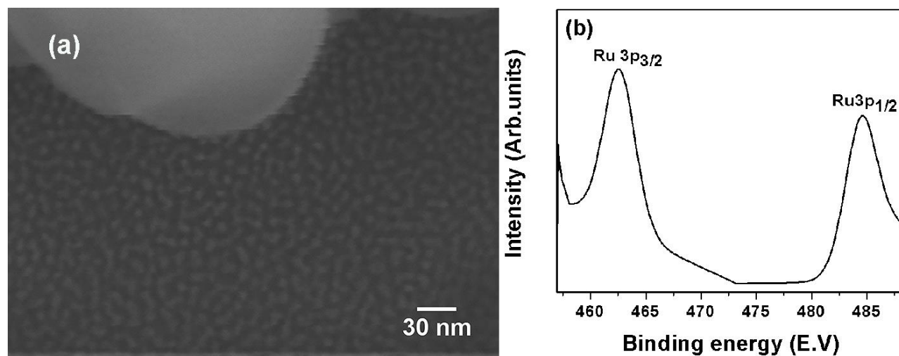
Figure 1. (a) SEM image of Ru nanoparticles grown on Si (100) after 200 cycles of PA-ALD growth at a substrate temperature of 230°C, (b) Ru 3p high resolution XPS spectra obtained from the same sample confirming the presence of Ru.
