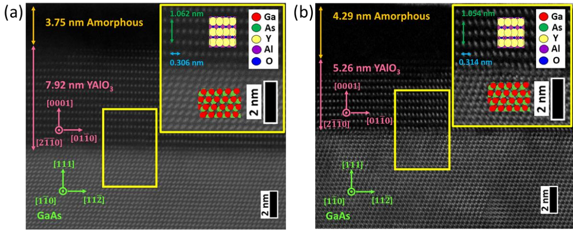
Fig.1 Cross-sectional STEM image of the samples utilizing (a) snl-ALD and (b) nl-ALD
