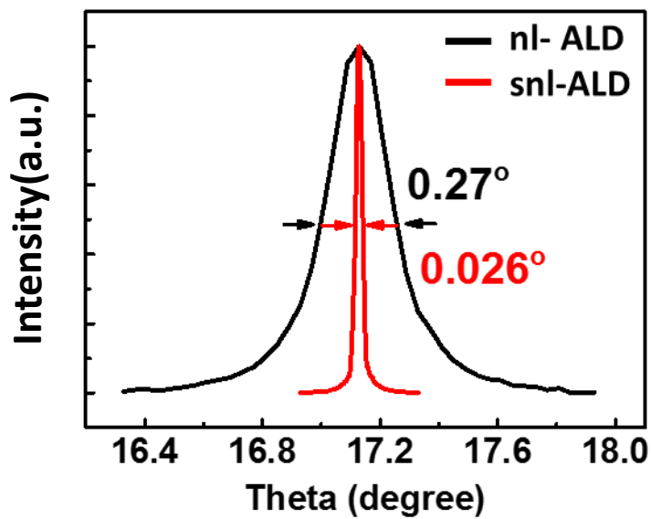
Fig.3 \theta -rocking scan of \text{YAIO}_3(0004) of the samples utilizing snl-ALD and nl-ALD
