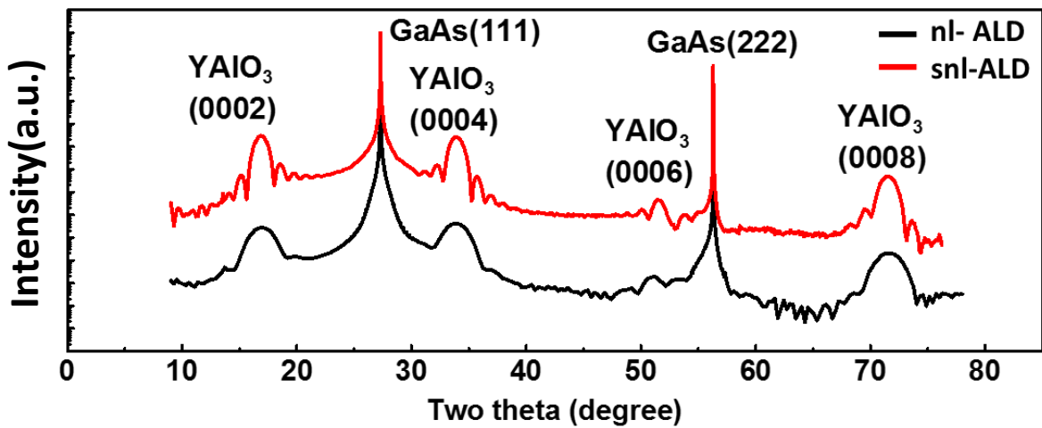
Fig.2 Radial scans along the surface normal of the samples utilizing snl-ALD and nl-ALD
