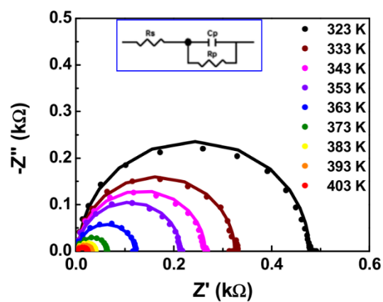
Figure S1. Impedance plots of lithium phosphate thin film deposited at 300 °C.
