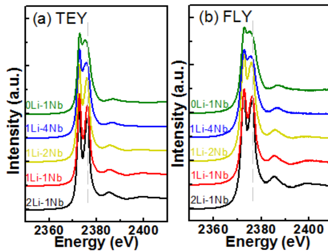
Figure S2. XANES of Nb L-edge in (a) total electron yield (TEY) mode and (b) Fluorescent Yield (FLY) mode.
