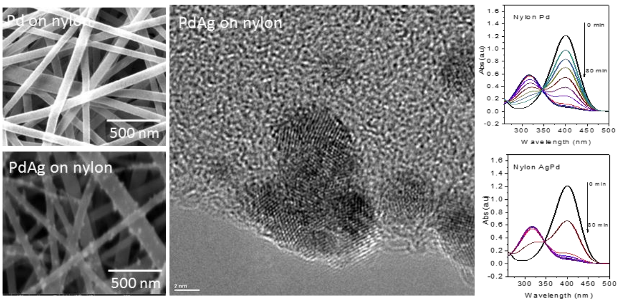
Figure 1. The morphology of the Pd and Pd-Ag loaded nylon nanofibers and its effective catalytic properties.
