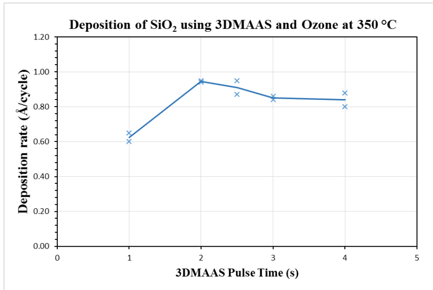
Figure 1. Saturation behavior of 3DMAAS at 350 °C.
