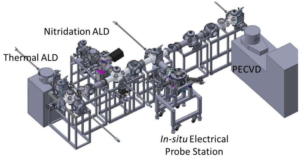
Figure 1. Schematic of the UHV cluster tool for in-situ electrical characterization
