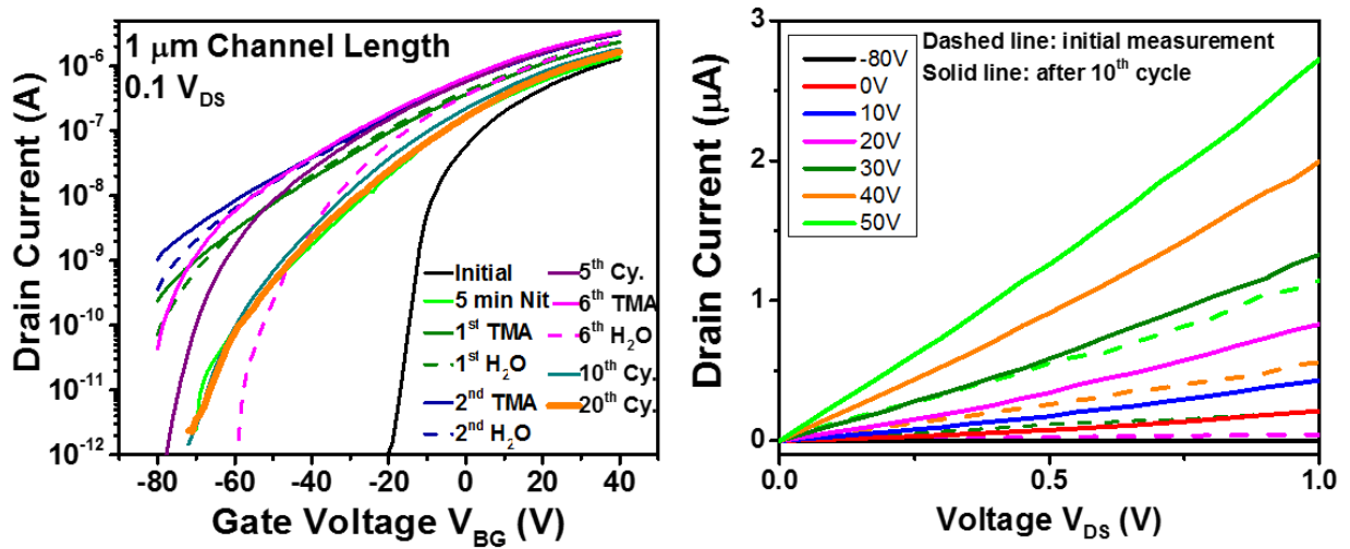
Figure 2. Transfer curves and output curves for nitrogen radical functionalization and ALD half-cycle
