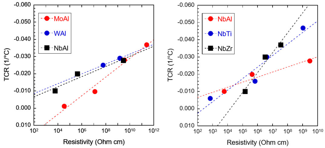
Figure 1. Thermal coefficient of resistance (TCR) for various ALD metal-metal oxide nanocomposites.
