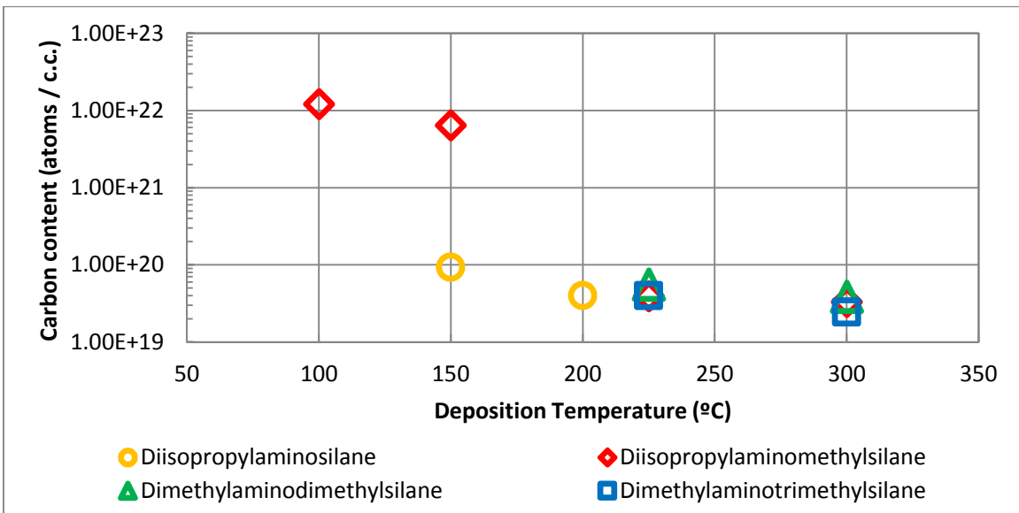
Figure 2. Carbon concentration of silicon oxide films deposited with different precursors at different temperatures, measured by SIMS.
