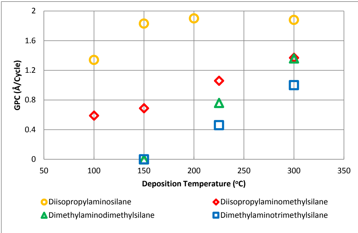
Figure 1. GPC of silicon oxide films deposited with different precursors at different temperatures.
