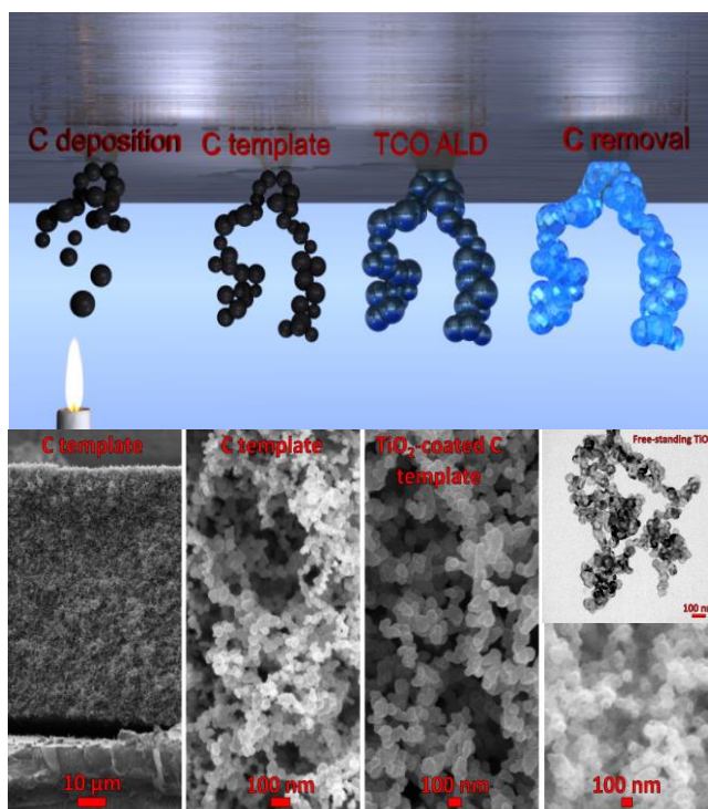
Figure 1: Schematic representation (top) and SEM/TEM images (bottom) of the processing steps for catalyst support preparation.
